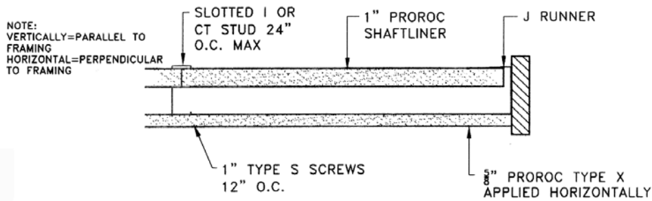
FIGURE 6—2-HOUR RATED HORIZONTAL CEILING
