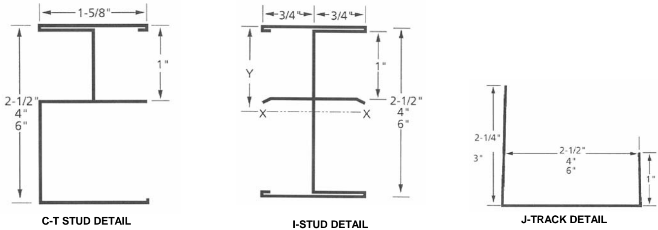
FIGURE 1—DIMENSIONAL DETAILS
