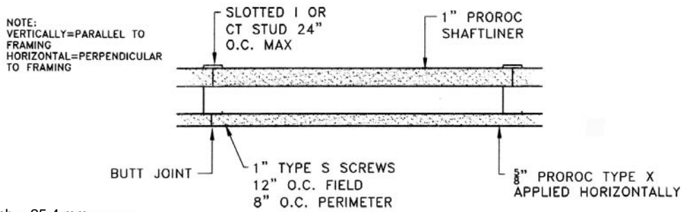
FIGURE 4—1-HOUR RATED PARTITION FINISHED ONE SIDE
