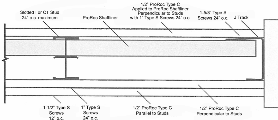
FIGURE 6—2-HOUR RATED HORIZONTAL CEILING
