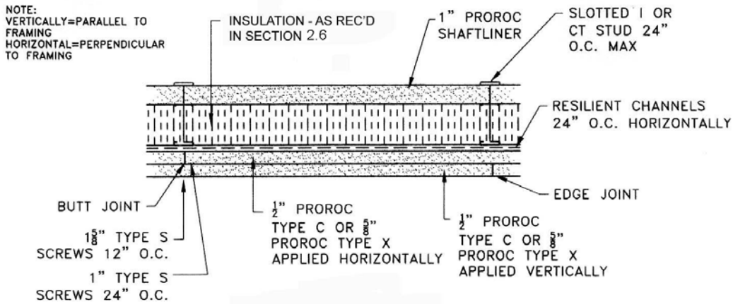
FIGURE 5—2-HOUR RATED PARTITION WITH SOUND CONTROL
