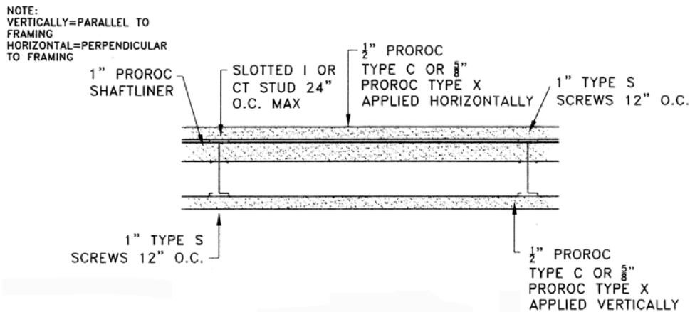
FIGURE 2—2-HOUR RATED PARTITION FINISHED ONE SIDE
